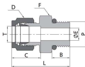
英制管-SAE/MS 外螺纹/Fractional Tube to SAE/MS Thread
