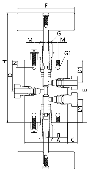
3通/2进 /2 stem manifold
