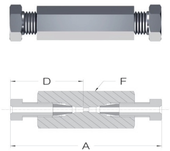
等径两通螺钉接头—BB Equal diameter two-way screw connector-BB
