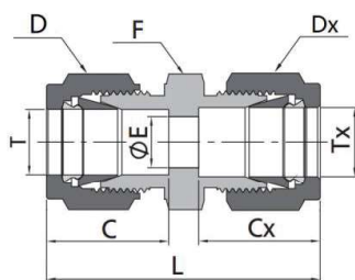
公制转英制管/Metric Tube to Fractional Tube
