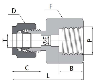
英制管-ISO平行内螺纹/Fractional Tube to ISO Parallel Thread
