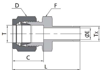
公制管—英制管/Metric Tube to Fractional Tube
