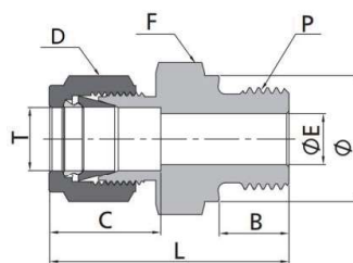
公制管-ISO平行外螺纹/Metric Tube to ISO Parallel Thread
