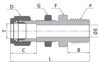
英制管-NPT 外螺纹/Fractional Tube to NPT Thread
