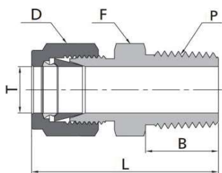
英制管-NPT外螺纹/Fractional Tube to NPT Thread
