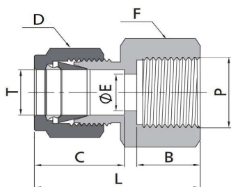
英制管-公制内螺纹/Fractional Tube to Metric Thread
