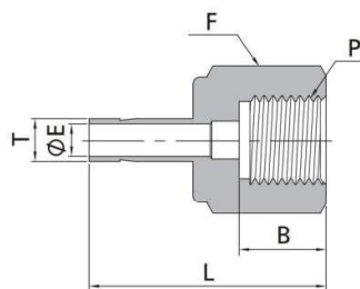
公制管-ISO平行螺纹/Metric Tube to ISO Parallel Thread
